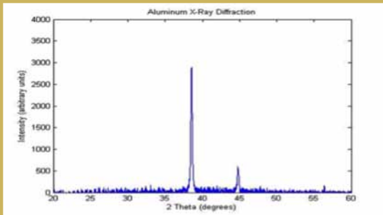
Figure 10: The MATLAB plot for the X-Ray Diffraction data of only the Al thin film obtained by aligning and subtracting the X-Ray Diffraction plot of just the silicon wafer from that of the silicon wafer with the Al thin film fabricated on it.
