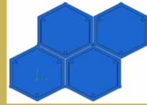
Figure 5: For FEM Analysis four unit cells represent the whole lattice due to symmetry
