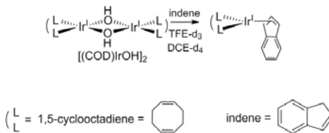
Figure 2: The reaction of the iridium dimer with indene.
